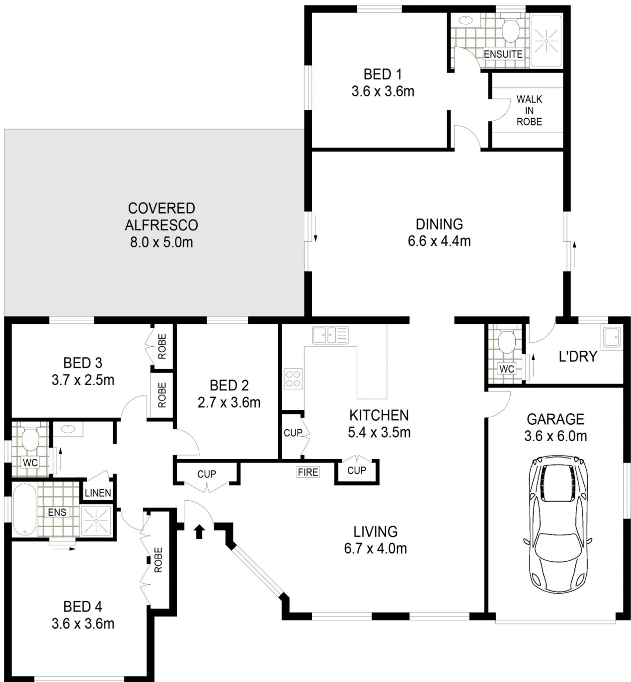
GROUND LEVEL
