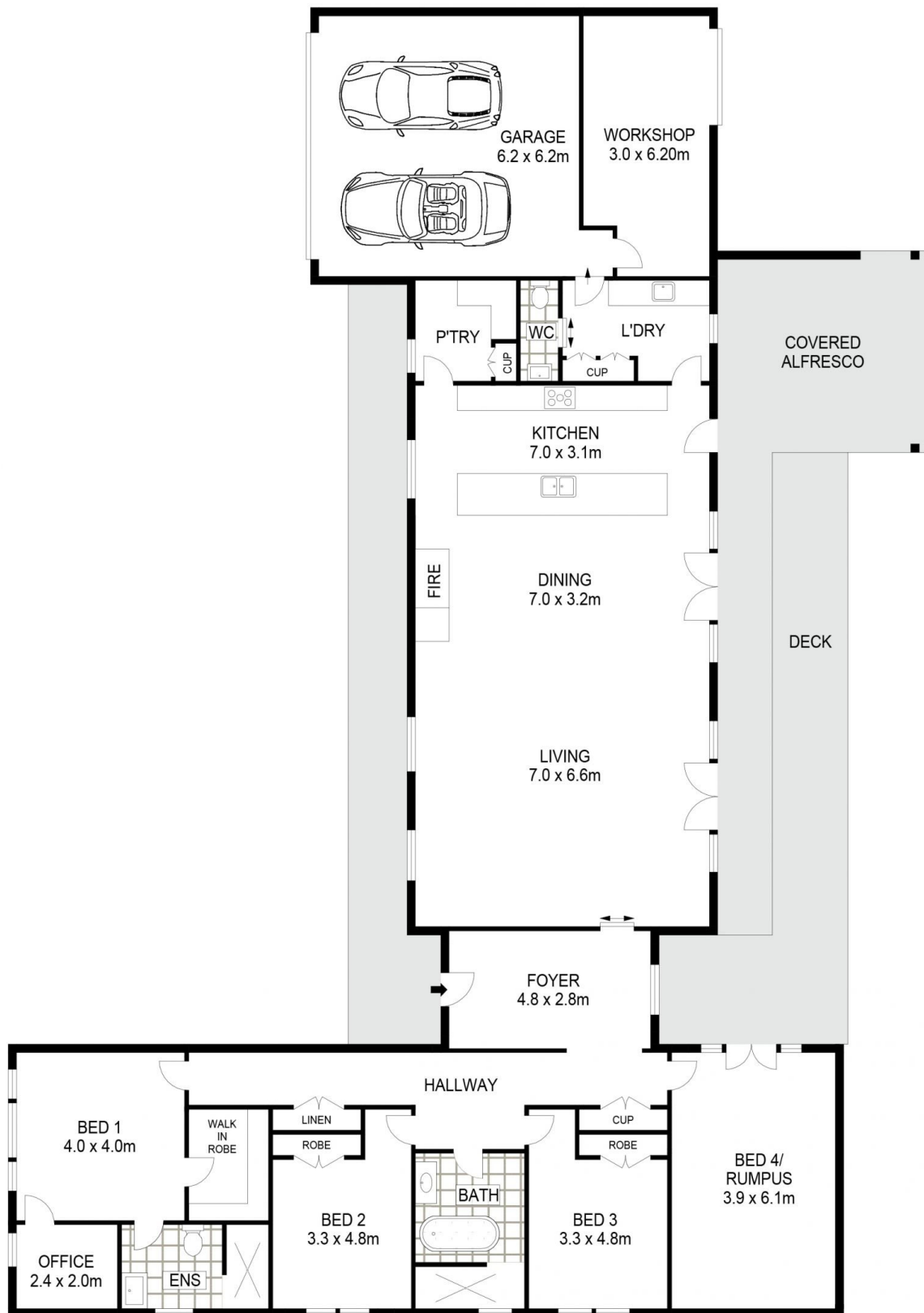
GROUND LEVEL
