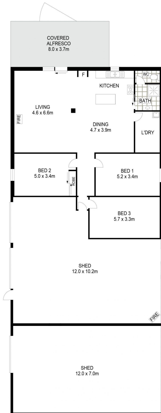
GROUND LEVEL
