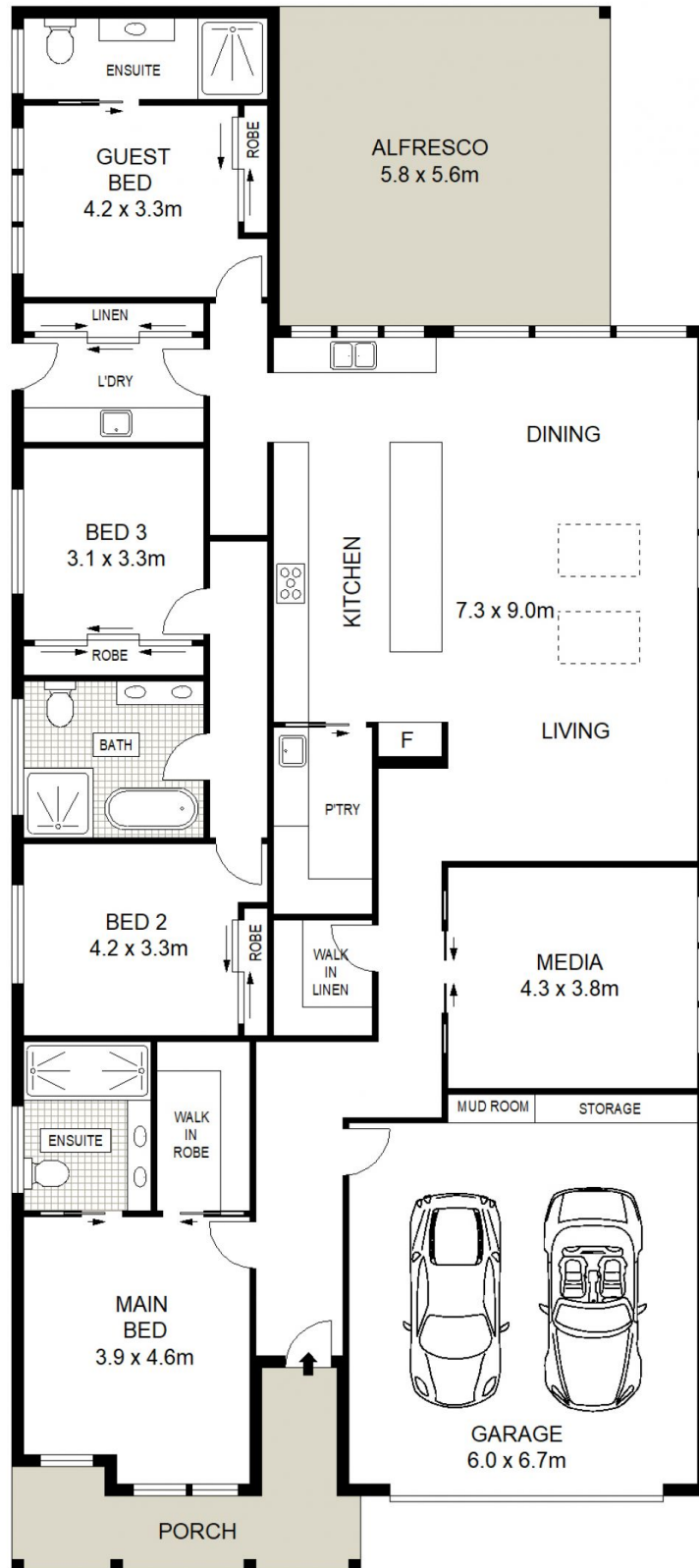
GROUND LEVEL
