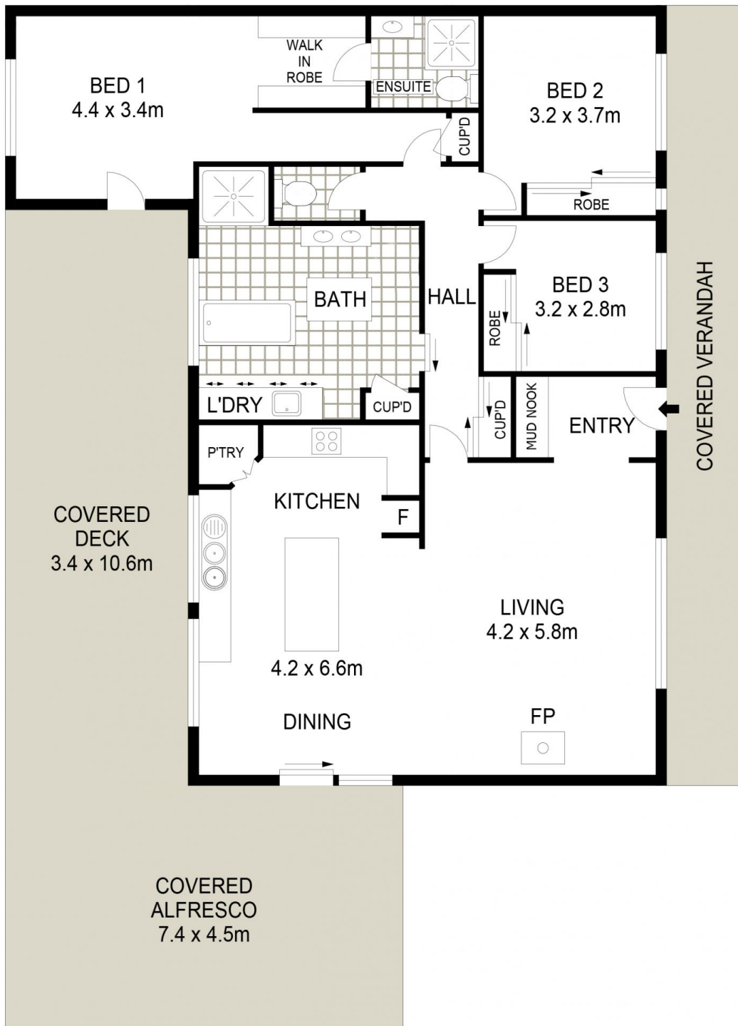
GROUND LEVEL
