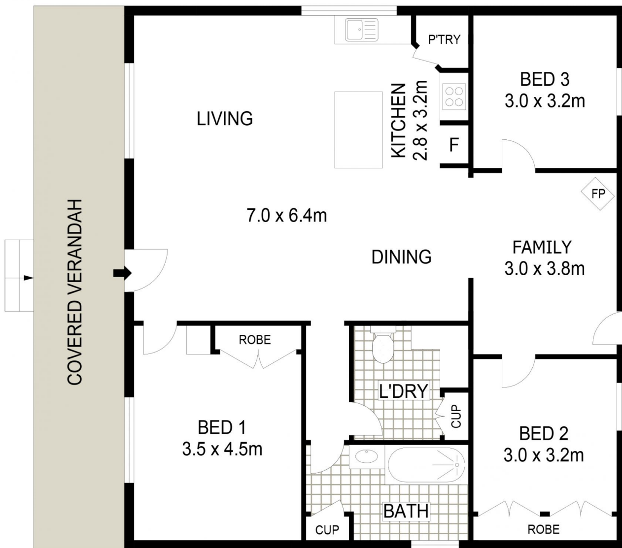
GROUND LEVEL
