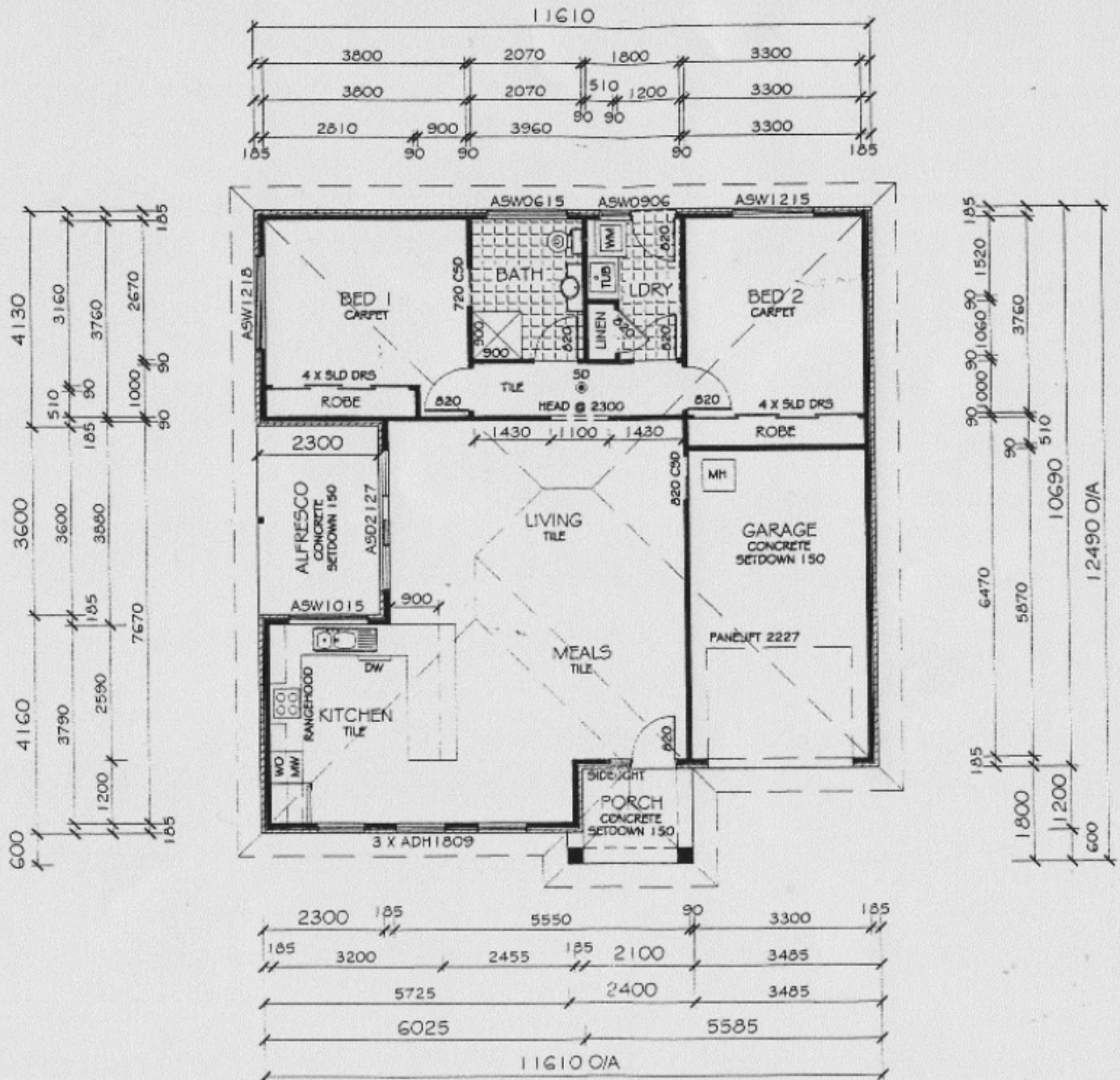
UNIT 2 FLOOR PLAN
